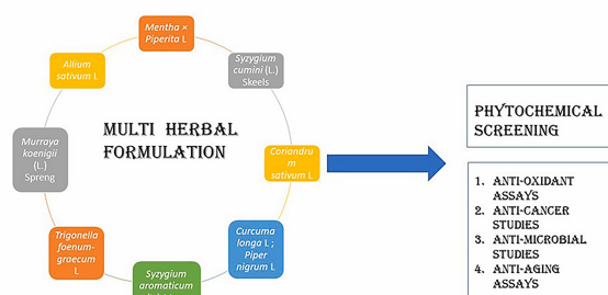
Figure 1: Schematic representation of the multi-herbal formulation comprising Mentha × piperita L., Syzygium cumini (L.) Skeels, Coriandrum sativum L., Curcuma longa L., Piper nigrum L., Syzygium aromaticum (L.) Merr., Trigonella foenum-graecum L., Murraya koenigii (L.) Spreng, and Allium sativum L. (6).
